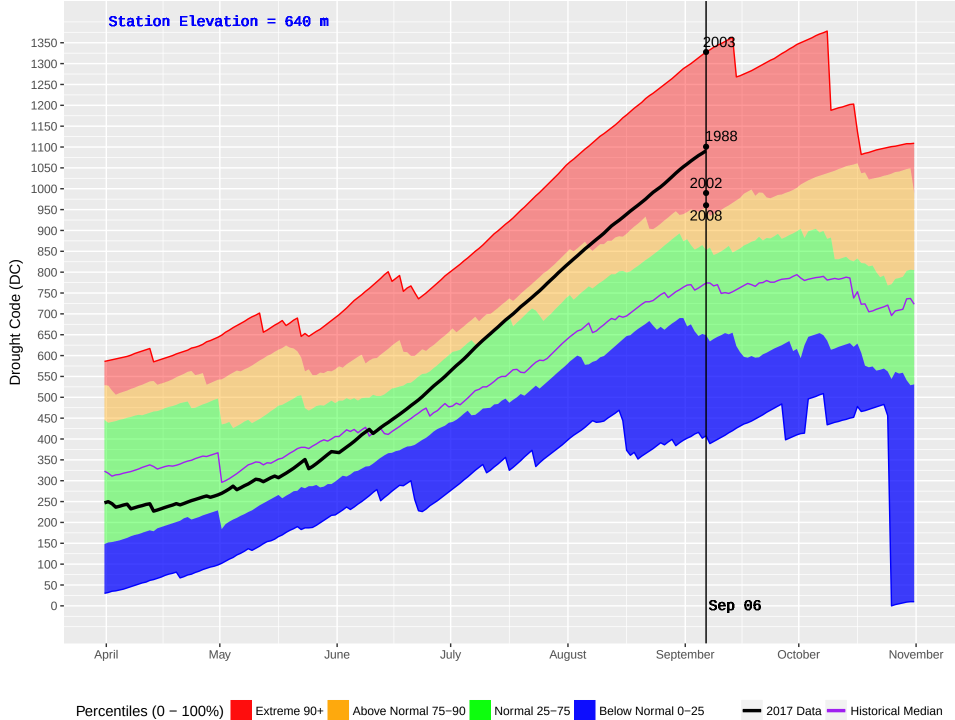
MERRITT HUB (294) : Historical (1978–2016) and Current (2017) Noon Drought Code (DC)
