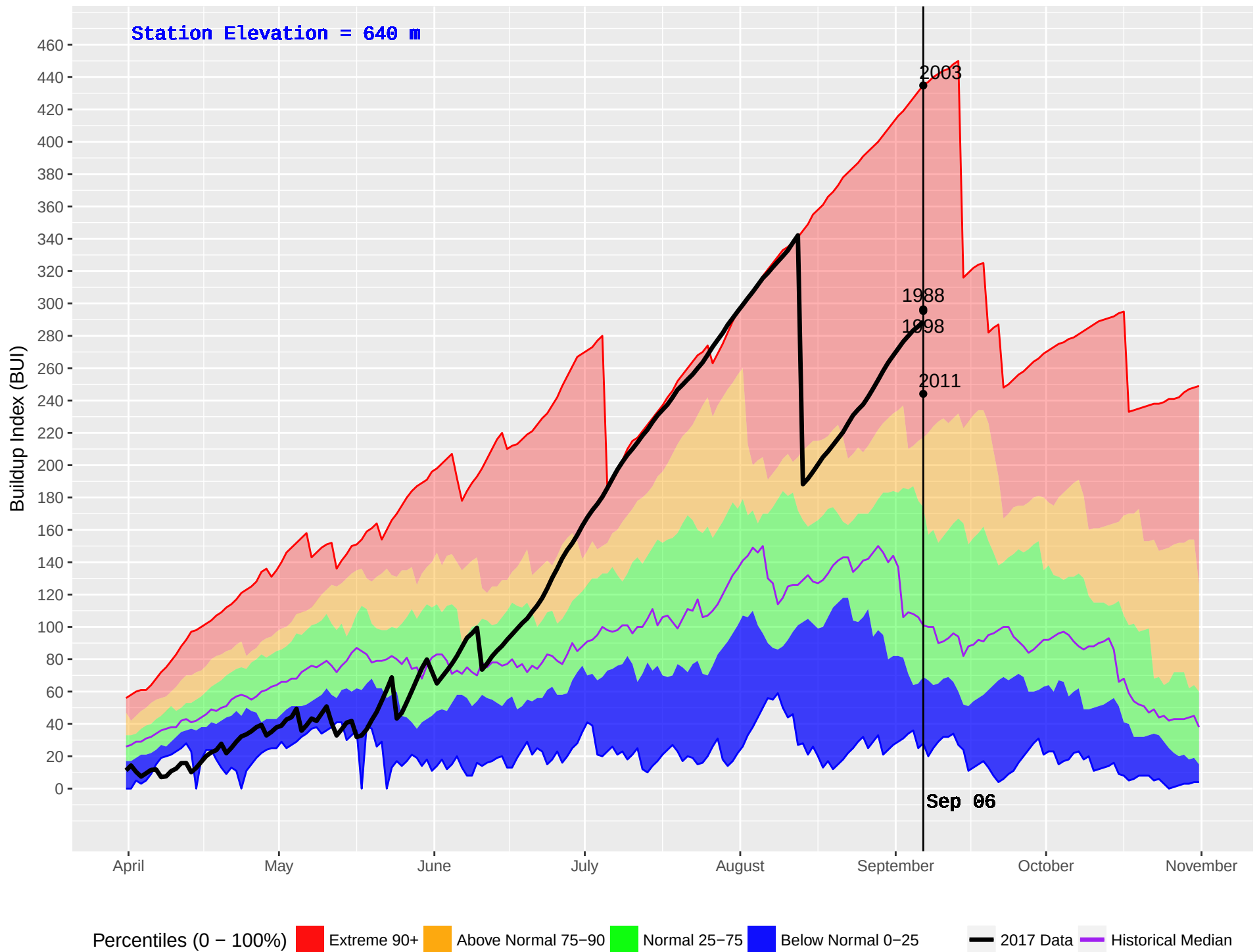
MERRITT HUB (294) : Historical (1978–2016) and Current (2017) Noon Buildup Index (BUI)
